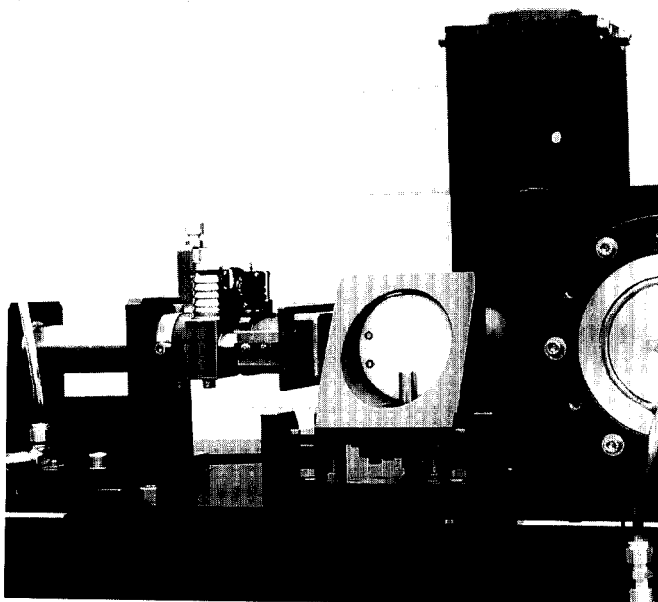
Fig. 2. The higher power (12kW) solid target station.
