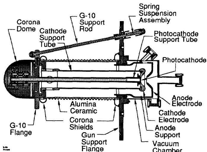
Figure 1. Schematic of the polarized electron gun.
