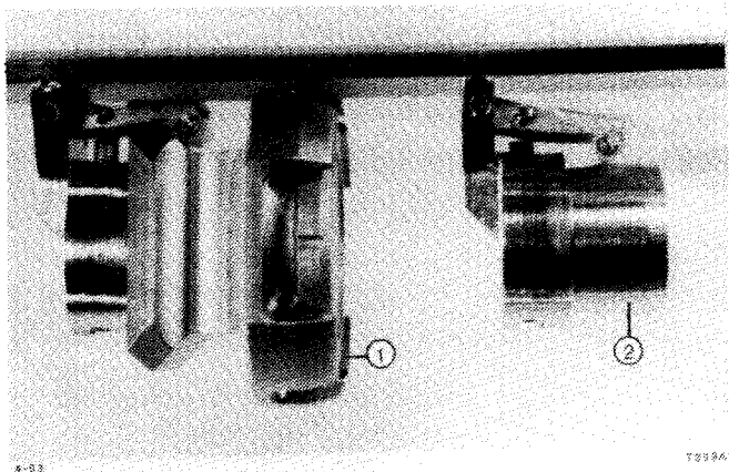
Figure 2. Photocathode carrier tray shows both a position occupied by a Mo wafer carrier (1) and an empty position (2).
