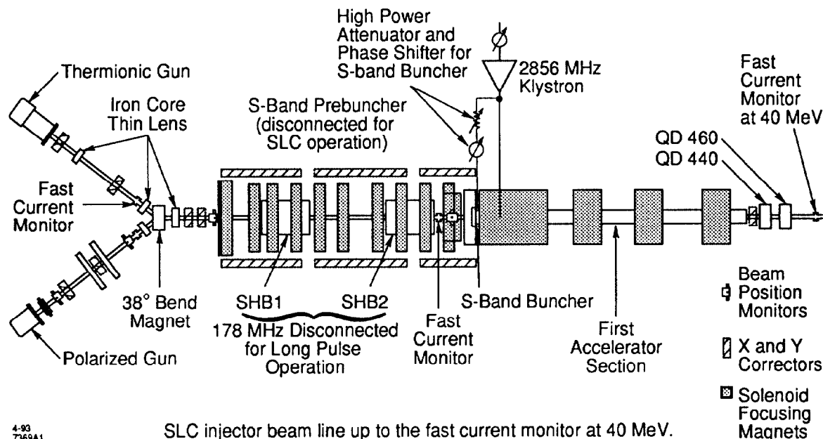
Figure 1. SLC injector beam line up to the fast current monitor at 40 MeV.
