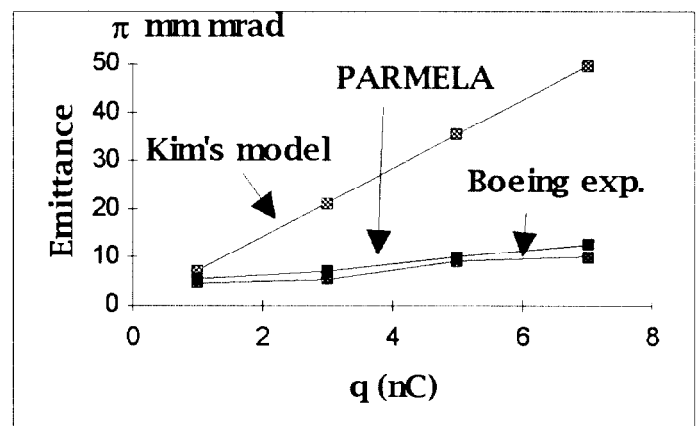
Fig. 3. Normalized rms emittance vs. charge for the Boeing PI compared to Kim's model.
