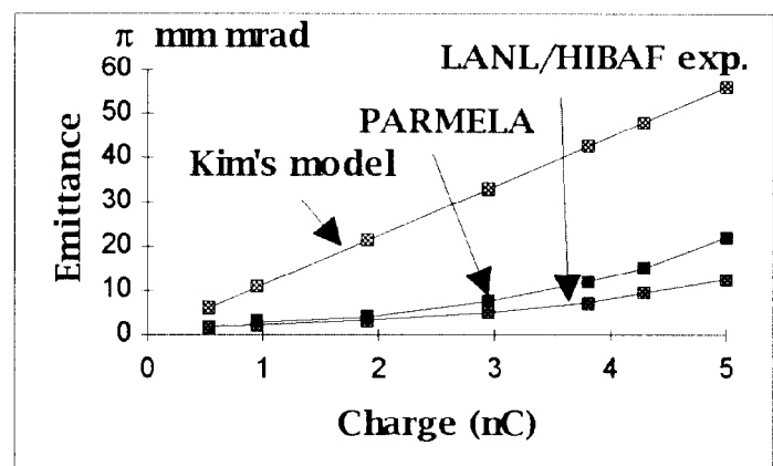
Fig. 4. Normalized rms emittance vs. charge for the LANL/HIBAF PI compared to PARMELA (with wake field) simulation and Kim's model.
