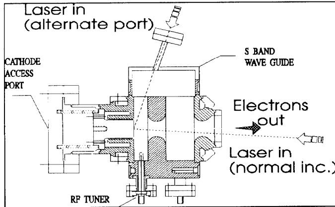
Fig. 1. Cross section of a 2.856 GHz, 1 1/2 cell PI.
