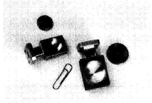
Figure 3 Photograph of the bunch length monitor cavities.
