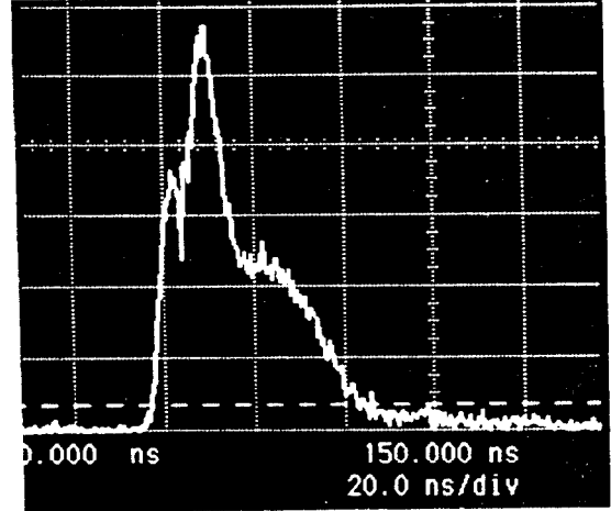
Figure 4 Measured signal from the 36 GHz monitor with \sigma_z = 1.8 \text{ mm} and 3 \times 10^{10} electrons. (Scale = 100 \mu\text{W} / \text{div.} )
