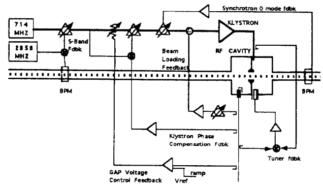
Figure 1. SLC damping ring rf system.
