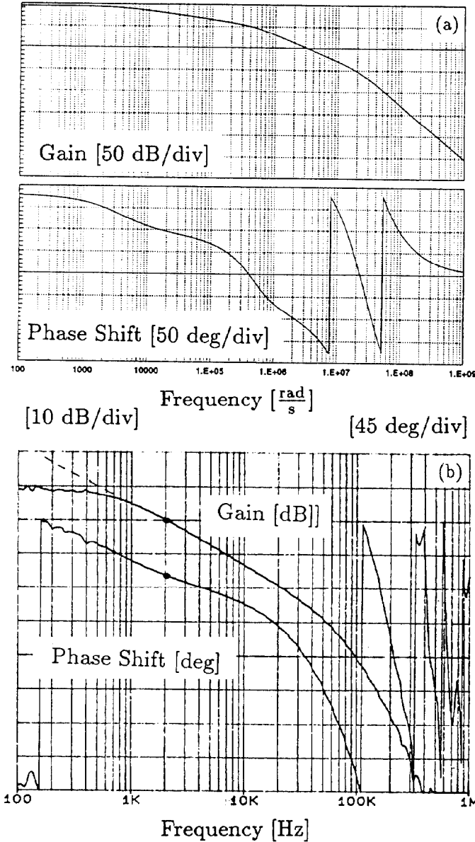
Figure 4. Calculated open loop response (fig. 4a) is compared with online measurement (fig. 4b)
