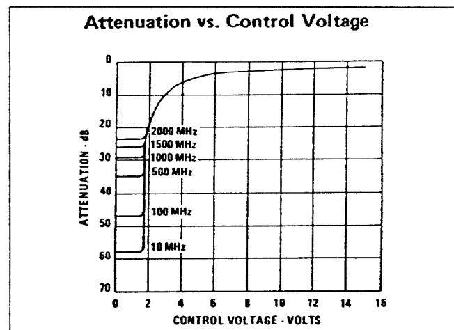
Figure 3. WJ-G2 diode characteristics.
