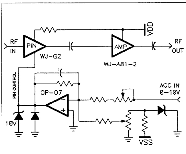
Figure 2. RF attenuator diagram.
