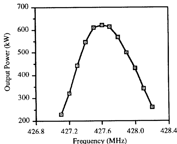
Figure 1. Frequency Response
