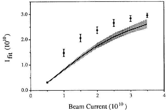
Figure 3. The fit value for the beam current from measured (circles) and simulated (solid line) BPM difference orbits as a function of the actual beam current. The shaded region is described in the text.
