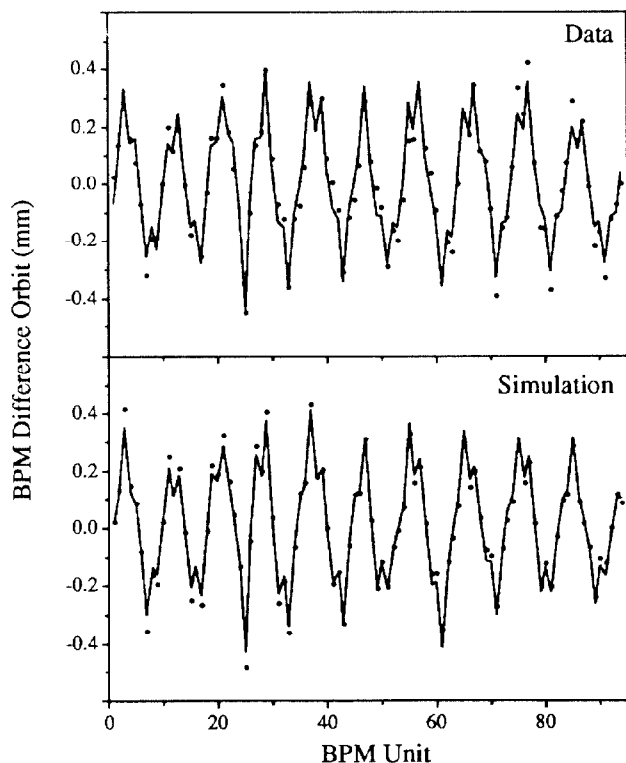
Figure 2. Measured and simulated BPM oscillations (circles) and the resulting fits (solid lines) for I=3.0 \cdot 10^{10} .
