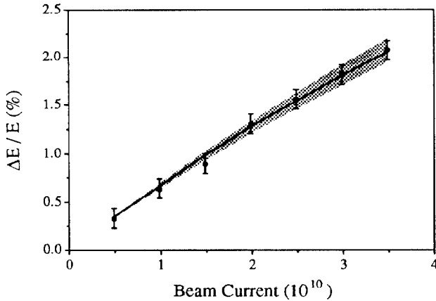
Figure 1. Measured (circles) and simulated (solid line) fractional energy loss as a function of beam current. The shaded region is described in the text.
