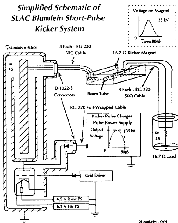
Figure 1. Short-Pulse Blumlein Kicker System.
