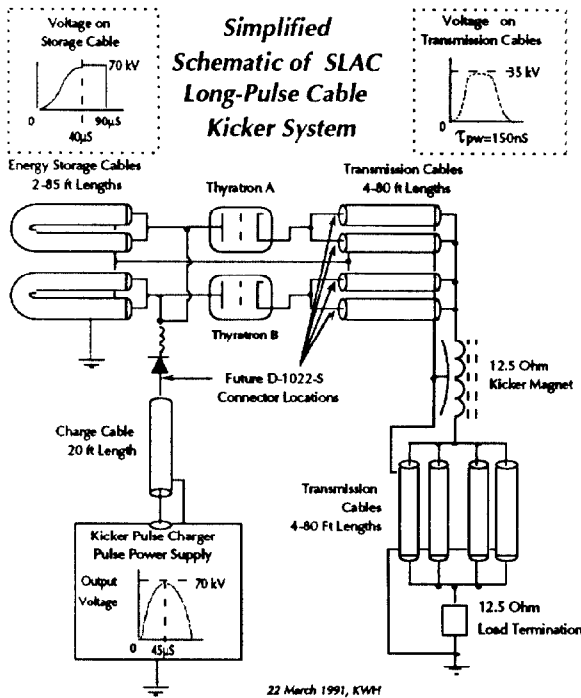
Figure 2. Long-Pulse Cable Kicker System.
