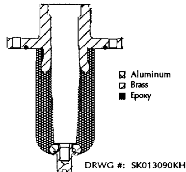
Figure 3. D-1022-S Connector for foil-wrapped RG-220.
