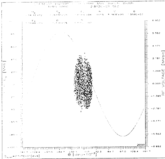
Figure 3: Main Ring bunch after slide-under transition crossing
