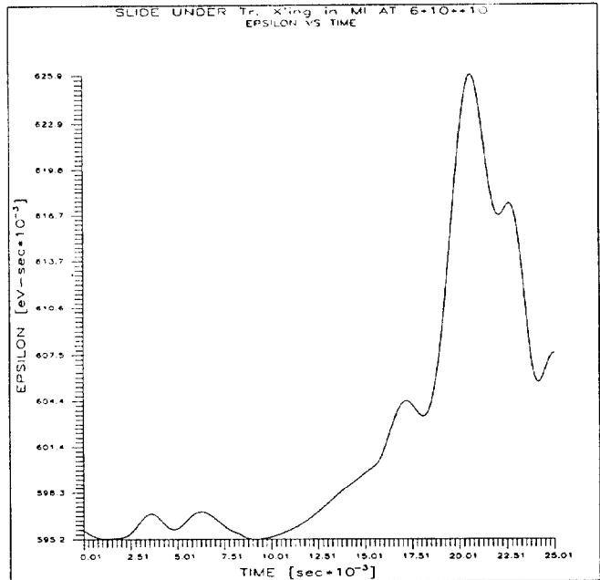
Figure 4: Longitudinal emittance ( 6\epsilon_{rms} ) vs. time for slide-under in MI
