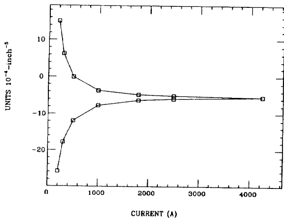
Figure 6: Current hysteresis of 12-pole moment
