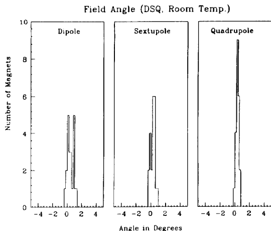
Figure 2: Field angle of coils in a DSQ package.
