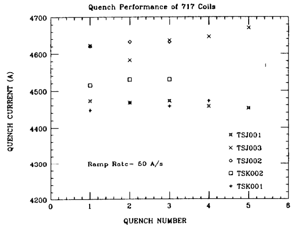
Figure 3: Quench performance of 717 coils at 21PSIA.
