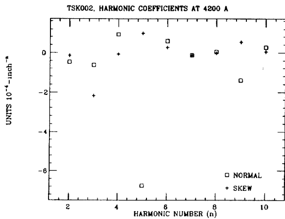
Figure 5: Harmonic moments of 717 coils TSJ002, NORMAL 12-POLE
