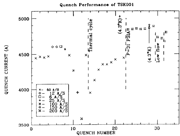
Figure 4: Quench performance of TSK001.
