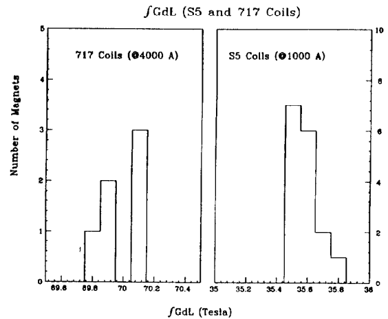
Figure 7: \int GdL for S5 and 717 coils
