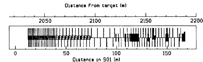
Figure 1. Layout of beam components in sector 1 and SLTR. Sector 1 ends at 100 m where SLTR starts. Quadrupoles are indicated by the lines which are either above (focussing) or below (defocussing) the horizontal axis. The only other elements indicated are accelerator sections (S01) and bend magnets (SLTR)
