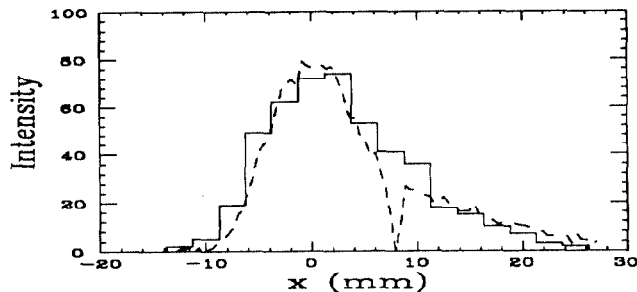
Figure 4. Horizontal beam profile in the SLTR where dispersion is large. Histogram: TURTLE; dashed curve: digitized profile screen measurement before earthquake. The dip in the dashed curve is due to the grid on the screen material.
