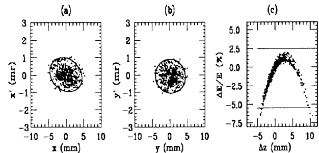
Figure 2. Six dimensional phase space from TURTLE at the end of sector 1.
