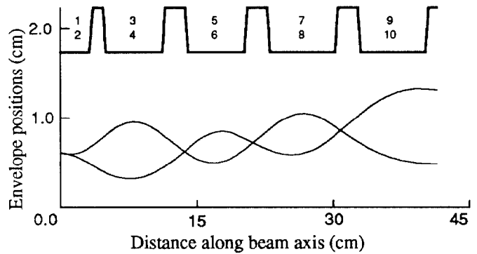
Fig. 6. Beam envelopes of a 84 mA He+ beam in the ESQ.
