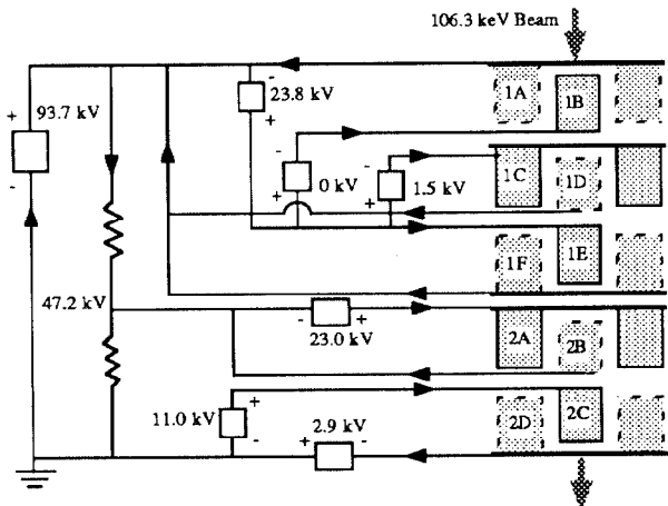
Fig. 2. Circuit diagram of the ESQ accelerator.
