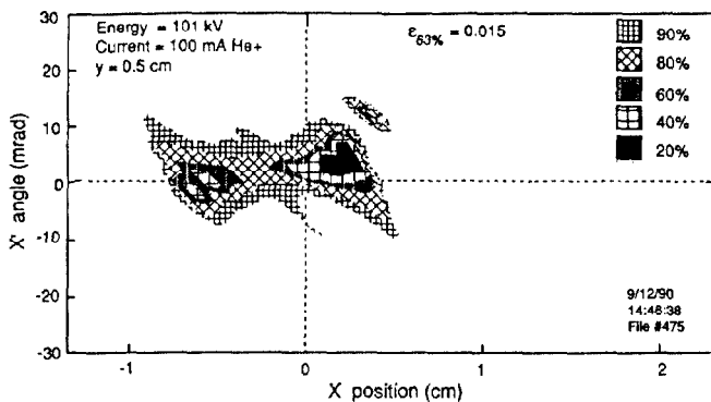
Fig. 3. Emittance Diagram of a 100 mA He^+ beam leaving the preaccelerator at 101 keV energy.
