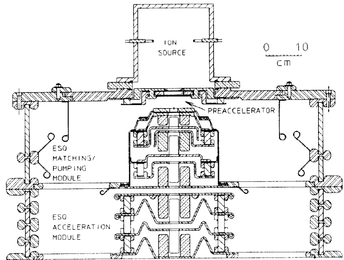
Fig. 1. Schematic Diagram of the prototype ESQ Accelerator
