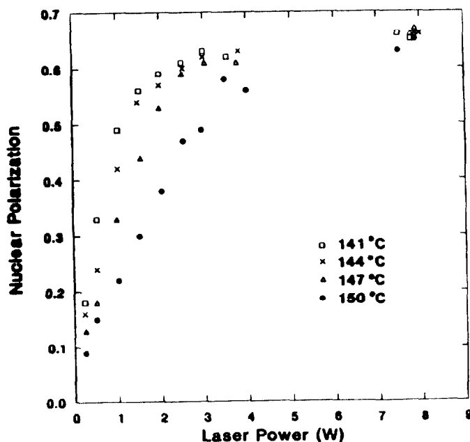
Figure 1: Nuclear polarization vs. laser power.
