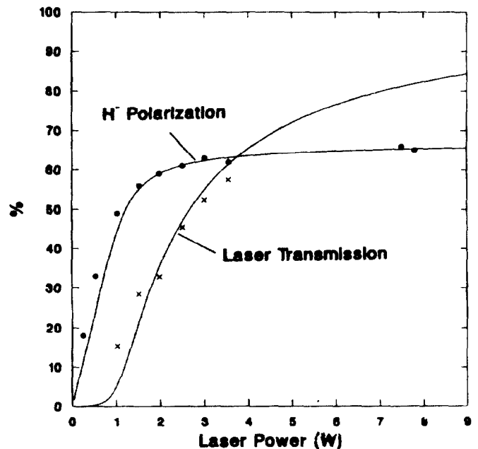
Figure 3: H^- polarization and laser transmission vs. laser power.
