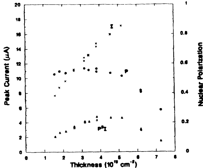
Figure 2: Nuclear polarization P , current I , and P^2I vs. target thickness.
