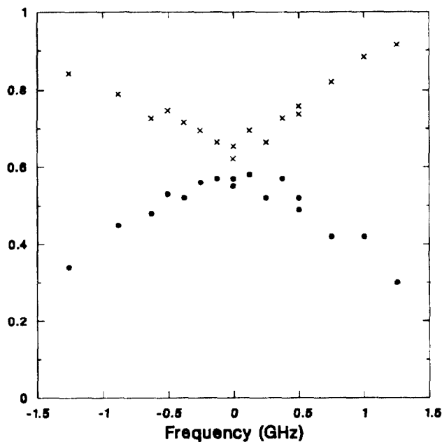
Figure 4: \text{H}^- polarization (circles) as a function of pump-laser detuning from K line center. The polarization remains high for detunings within \pm 0.01 \text{ cm}^{-1} ( \pm 300 MHz). The transmission of the laser beam through the target (crosses) is an operationally useful relative indication of polarization.
