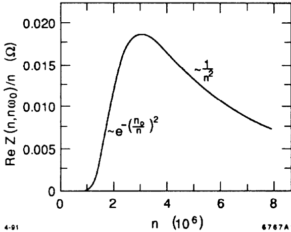
Figure 1. \text{Re } Z(n, n\omega_0)/n versus n for the parallel-plate model, R = 149.5 m, h = 2 cm.
