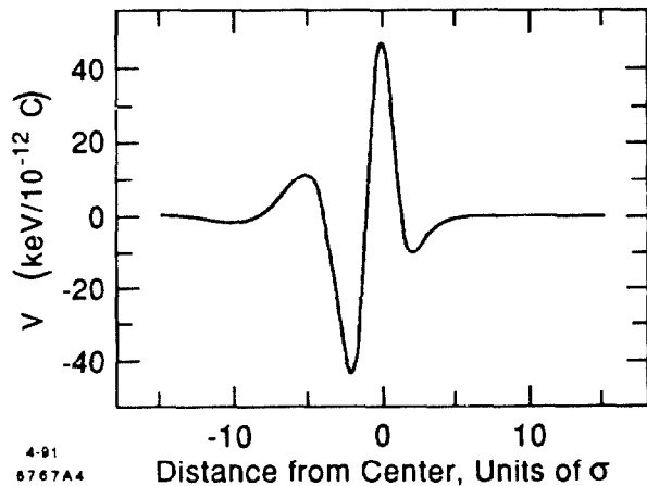
Figure 3. Wake voltage per turn for the parallel-plate model, R = 149.5 m, h = 2 cm, bunch length \sigma = 61 \mu\text{m} .
