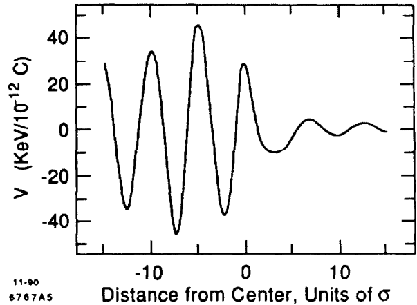
Figure 4. Wake voltage per turn for the toroidal chamber, R = 149.5 m, h = w = 2 cm, bunch length \sigma = 61 \mu\text{m} .
