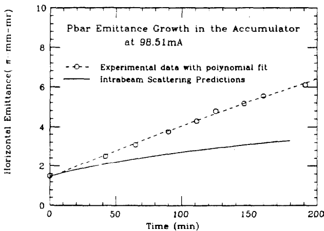
Figure 1. The Horizontal emittance versus time.
