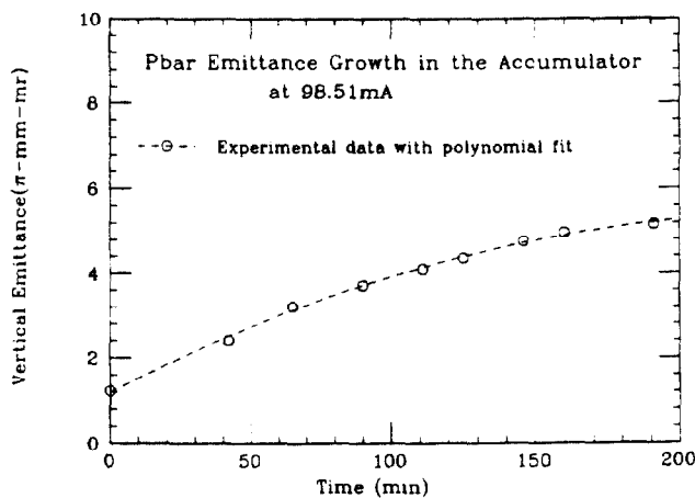
Figure 2. The vertical emittance versus time.
