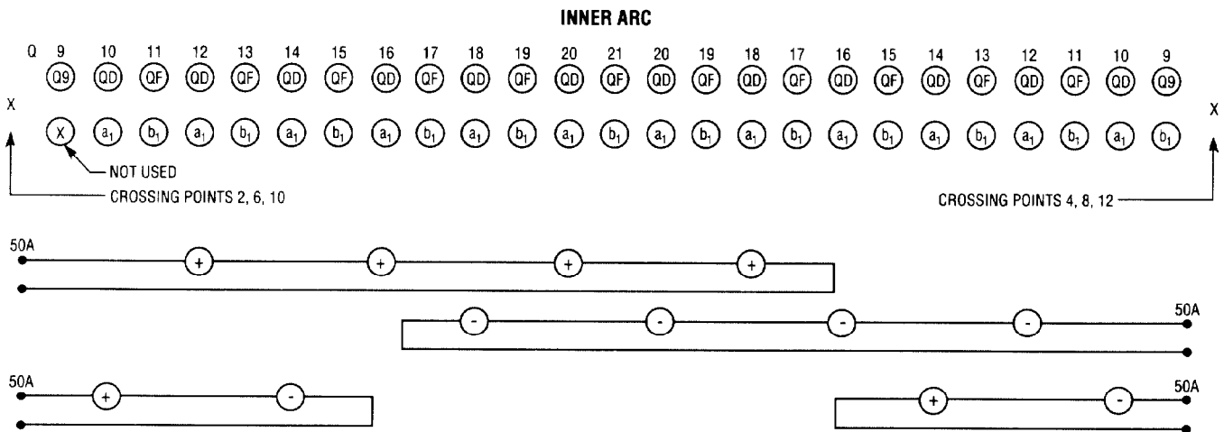
Fig. 2: Arc corrector configuration.
