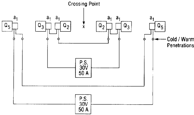
Fig. 1: Insertion corrector configuration.
