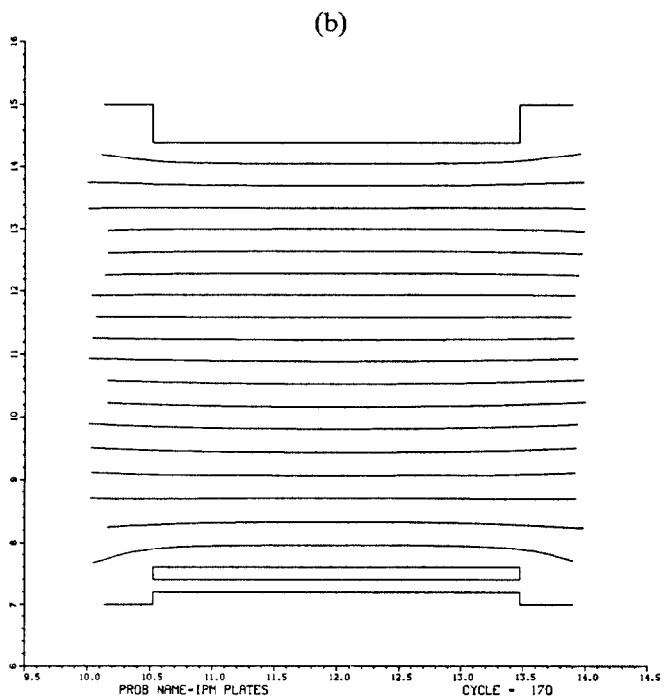
Fig. 2. Poisson calculations of equipotential lines in the ionization profile monitor collection volume. These views are cross-sections of the collection volume and show the characteristic U-shape of the electrodes. Each electrode lip is one quarter the length of the electrode. In both views the -70 kV electrode is at the top and the ground electrode at the bottom; the voltage between potential lines is 3.5 kV. Scale is in cm. In (a), the input face of the microchannel plate detector is the upper dotted line. This face is held at -2 kV by the bias power supply. The characteristic dual plate capacitor potential lines have given way to flat potential lines due to the lips on the electrodes. In (b), a magnified view of the collecting volume shows that its electric field is essentially constant. Here the micro-channel plate detector is the rectangle above the lower electrode.
