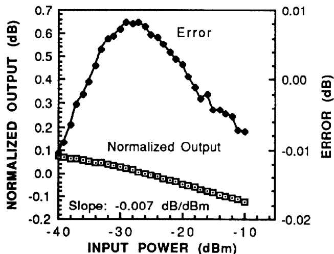
Figure 5. Error and normalized output curves for the 0-dB line of Figure 3.
