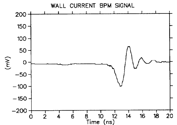
Figure 5: Beam signal picked up by the wall current BPM
