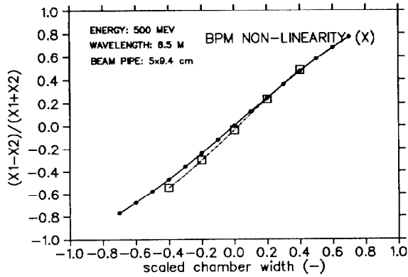
Figure 2: BPM Transfer Function (X)
