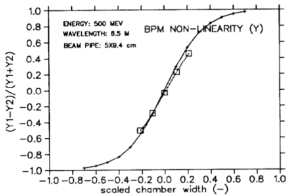
Figure 3: BPM Transfer Function (Y)
