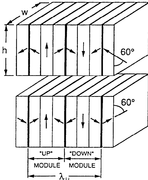
Figure 3. 6-block PPM construction.
