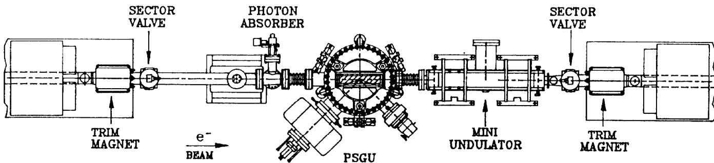
Figure 2. Layout of X13 insertion straight section.
