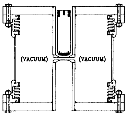
Figure 1. PSGU vacuum chamber concept.
