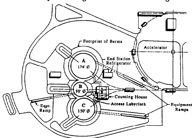
Figure 3. Beam switchyard configuration showing orientation of end stations and BSY transport lines.
