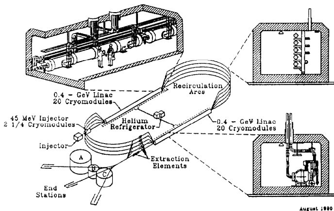
Figure 1. Machine and transport system configuration.
