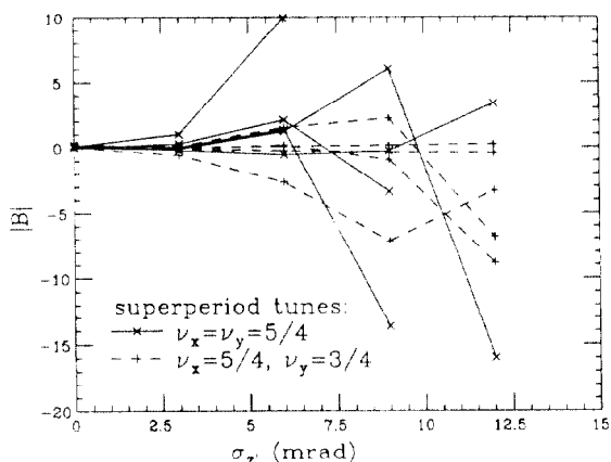
Figure 2. Coupling parameter dependence on rms arc element roll for randomly selected machines for each of two test tunings of the 3645 MeV line.
