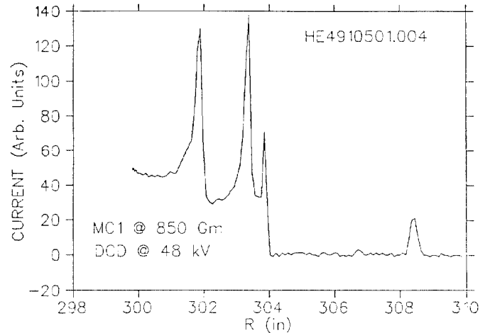
Fig. 5. Radial beam density scan in the cyclotron, showing separated beam downstream of the magnetic channel.
