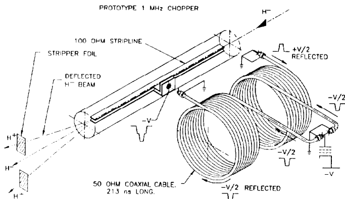
Fig. 2. Schematic diagram of rf beam chopper.
