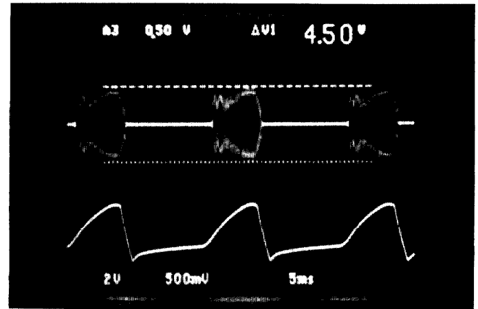
Fig. 3. High power operation of rf cavity using perpendicularly biased ferrite. The top trace shows voltage at the accelerating gap (dashed lines indicate 65 kV), the lower trace the bias power supply voltage.
