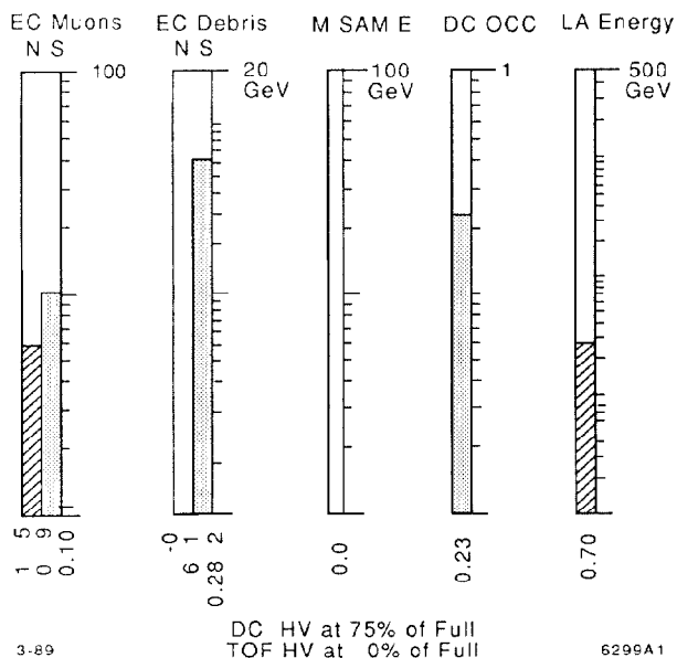
Fig. 4. Bargraph display available in the Mark II and SLC control rooms. Each bar represents a particular background measurement. The status of certain detector systems are displayed at the bottom. Not shown are various error and status messages that are available on the same page.
