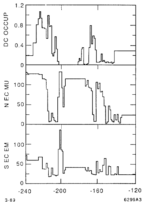
Fig. 5. Background history display. Each plot shows a different measurement versus time. The time scale is selectable, as is the amount of averaging done. About 40 different quantities are available for plotting.
