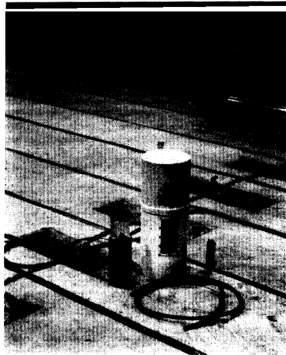
Fig. 1. The four types of dedicated monitors. The large white cylinder in the center is a BSOIC, with a PIC to the left and a PT to the right. In front is a short length of PLIC cable.
