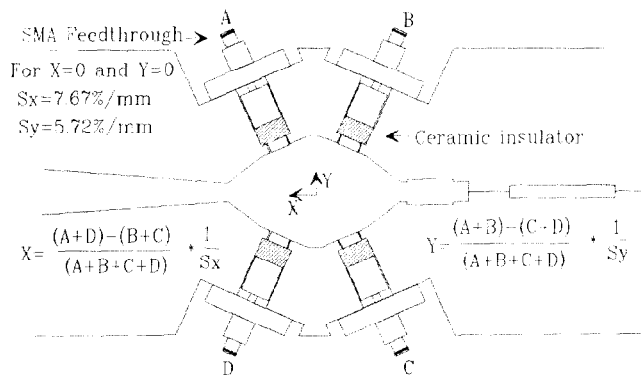
Fig. 1 Sector arc chamber showing button installation
