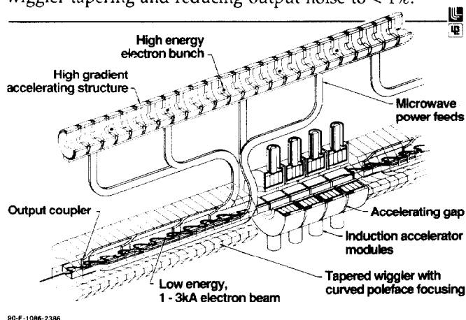
Figure 1. FEL/TBA Configuration
