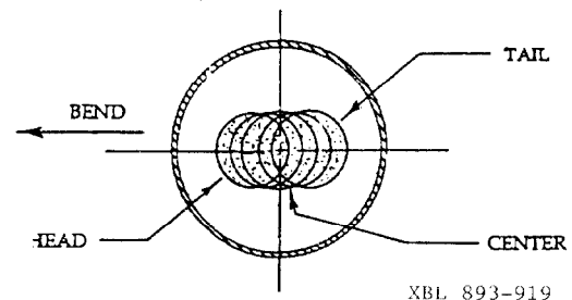
Fig. 2 Beam Dispersion in 180° Bend
