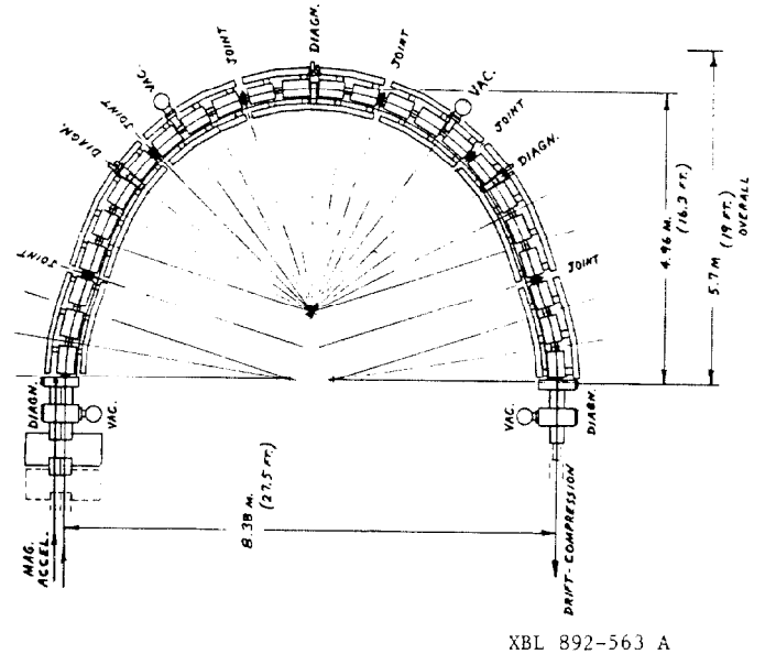
Fig. 1 Bend section plan view.
