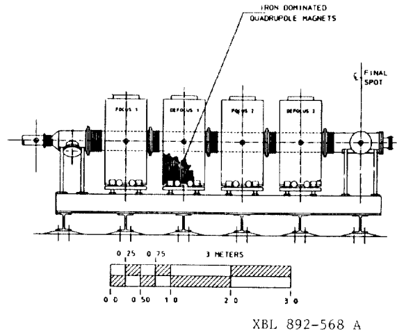
Fig. 5 Final Focus Side View
