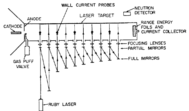
Fig. 1. Experimental Configuration.
