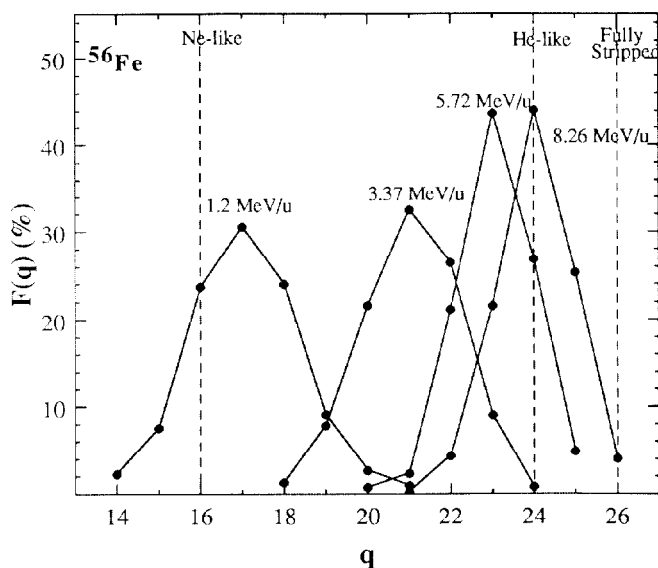
Figure 1. Measured charge state distributions for ^{56}\text{Fe} at 1.2, 3.37, 5.72, and 8.26 MeV/u. The incident charge was +4 for the 1.2 MeV/u measurement and +17 for the higher energies. The vertical dashed lines correspond to the fully stripped, He-like, and Ne-like ions.
