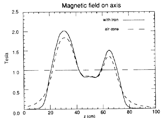
Fig. 4. A plot of the magnetic field on axis for the GEGR at design field. Dotted line shows an air core calculation and the solid line shows a calculation including the effect of the iron yoke. The broken line at 1.0 Tesla indicates the resonant B field at 28 GHz.
