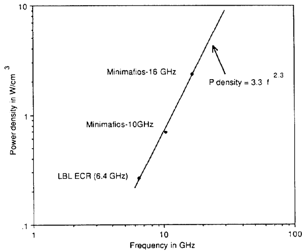
RF power density versus frequency in ECR sources
