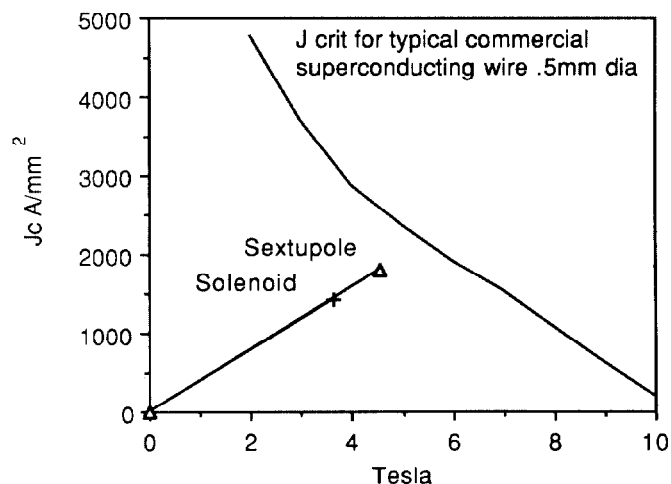
Fig. 5. A plot of the critical current in the superconductor for 0.5 mm NbTi wire. The load lines show the operating points for the sextupole and solenoid in their combined fields.
