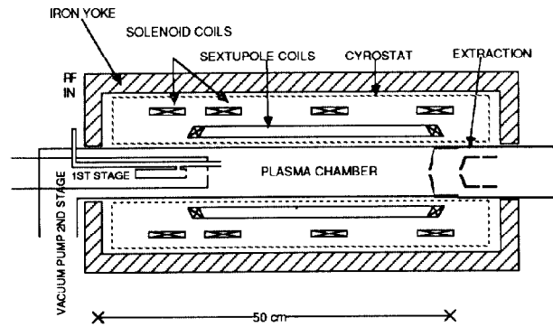
Fig. 3. An elevation view of the GEGR showing the main components. The cryostat is schematically indicated by the dotted lines.
