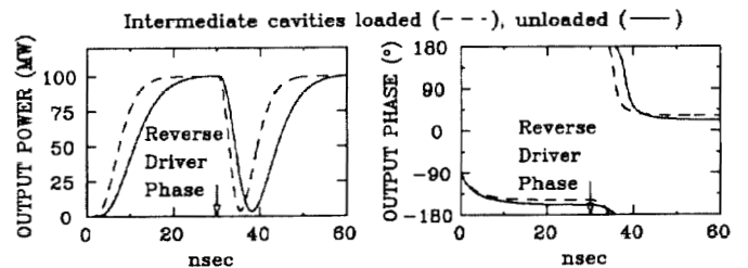
FIG. 4. Transient analysis of a 100-MW, 11.424-GHz five-cavity conventional klystron design for RF pulse compression. In this linear calculation, the RF generator is switched on at 0 nsec in the presence of a DC beam. The generator phase is reversed at 30 nsec, after the switch-on transient has subsided. Dashed curves show that improved risetime is obtained by adding external loads with Q_e = 150 to the gain cavities. Input Q_e = 190 . Output Q_e = 26 . The klystron cavity frequencies without beam are tuned to 21, 18, 40, 500, and 20 MHz, respectively, above 11424 MHz. The DC, 510 A, 440 kV beam detunes the cavities by -21 MHz and loads them with Q_b = 210 . For the five cavities, R/Q = 36, 36, 36, 39, and 20\Omega , respectively. Intercavity spacings are 6, 6, 8, and 3 cm.
