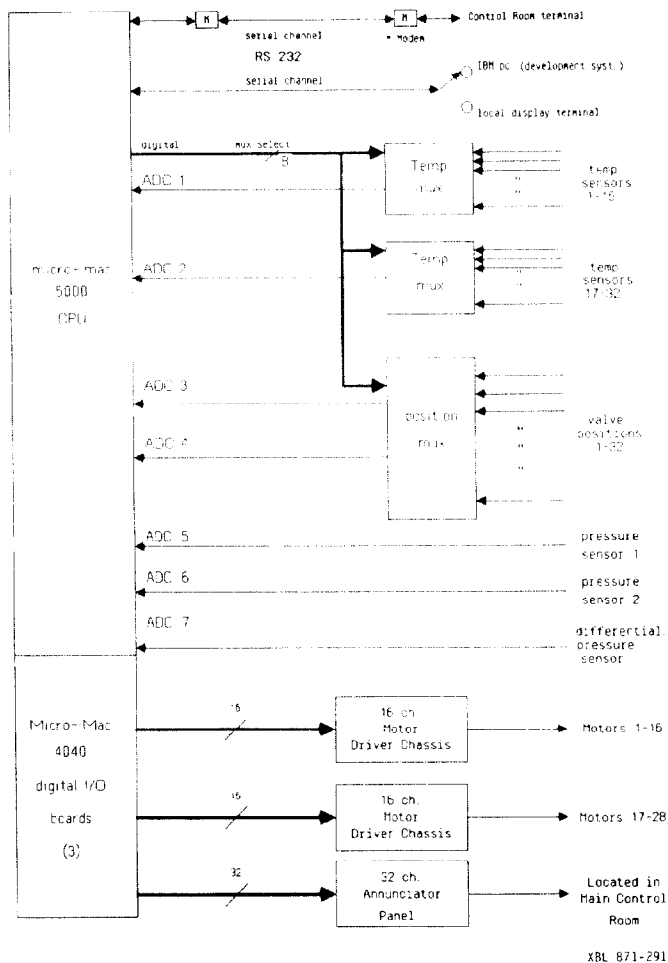
Fig. 3 - Electrical schematic
