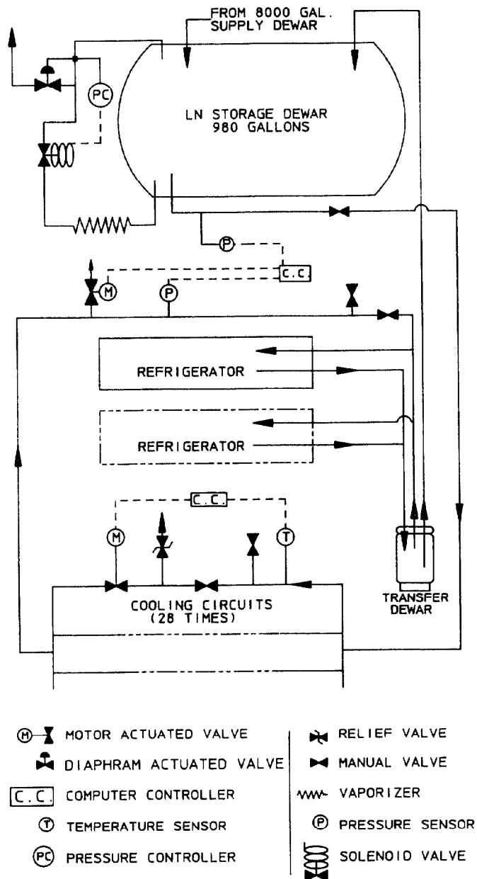
Fig. 1 - Plumbing schematic
