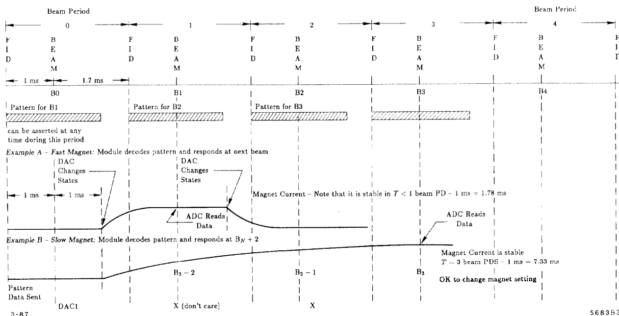
Figure 1. Timing Chart
