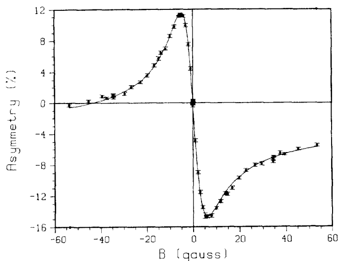
Fig. 2. Experimental data and fitted function for the asymmetry 12-34/12+34 as a function of the transverse magnetic field B. A positive asymmetry means that more counts are present on the +X side of the channel.
