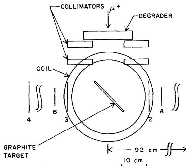
Fig. 3. Geometry for measurement of beam polarization. 83 MeV/c \mu^+ enters from above, traverses 3.6 cm polyethylene degrader, is collimated with Cerrobend pieces, and enters an ATJ graphite target. Asymmetries 12-34/12+34 and 12A-34B/12A+34B are measured as a function of the field B. Counters 1 and 4 are located each 92 cm from the beam axis. Counters are 1/16 inch thick. Counter 1 is on the +X side of channel, and positive field B is along +Y or out of the paper and precesses \mu^+ toward -X giving negative asymmetry.
