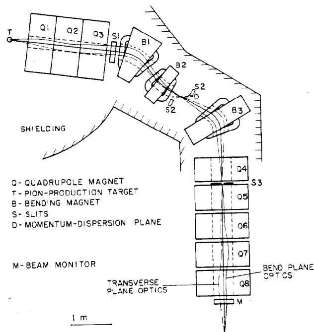
Fig. 1. LAMPF biomedical channel configured for backward-decay muon beams. The decay region is between B2 and B3 and extending inside B3.
