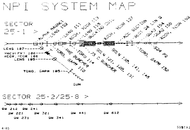
Fig. 3. Computer display of the NPI system showing the injector in Sector 25-1 and the special NPI quadrupole lattice in Sectors 25-2 through 25-8.
