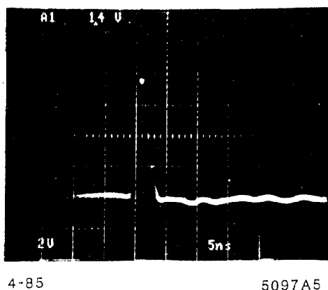
Fig. 5. NPI gun current pulse for SPEAR storage ring. Vertical \sim 250 mA/cm; horizontal 5 nsec/cm.
