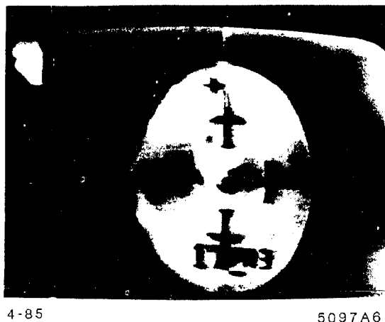
Fig. 6. SPEAR electron beam from NPI on profile monitor at entrance to storage ring. Beam spot appears flat on one side because of a burned spot on the screen.
