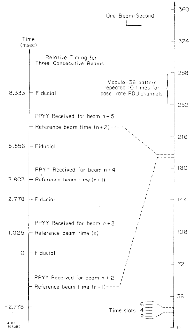
Fig. 2. Relative timing diagram.
