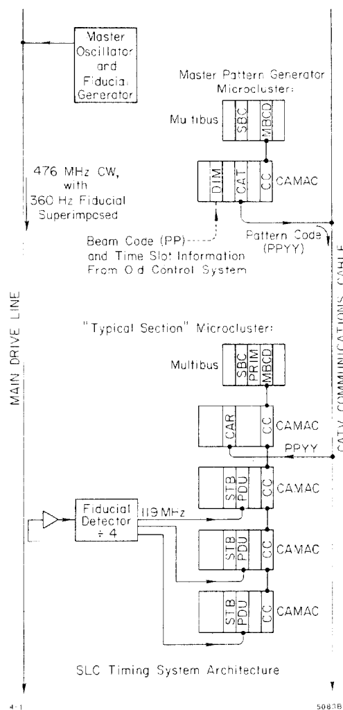
Fig. 1. The timing system architecture. CAR = Cable Access Receiver; CAT = Cable Access Transmitter; CC = SLC Serial Crate Controller; DIM = Digital Input Module; MBCD = Multibus CAMAC Driver; PDU = Programmable Delay Unit; PRIM = Pattern Receiver Interrupt Module; SBC = Single Board Computer (Intel iSBC 86/30); STB = Simple Timing Buffer.
