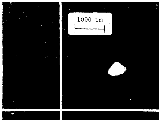
Fig. 6. Beam spot on a profile monitor at 6.5 GeV near a 340 \mu\text{m} fiducial hole. The crossed lines indicate the digitized scan lines.
