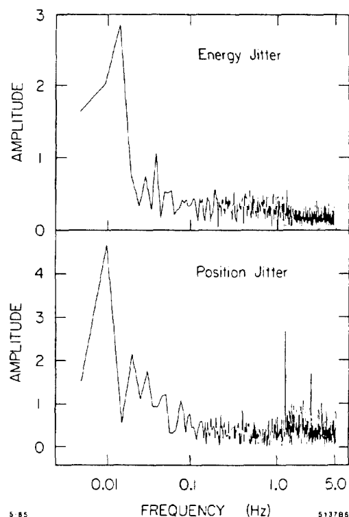
Fig. 8. Spectra of position and energy fluctuations.
