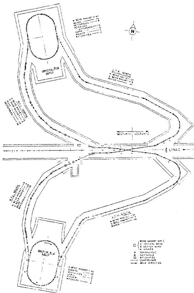
Figure 1. Layout of the Damping Ring Complexes
