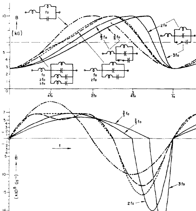
Fig. 3. B and \dot{B} values for various magnet excitations.
