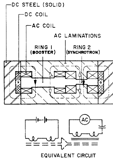
Fig. 2. Two rings utilizing one core structure.
