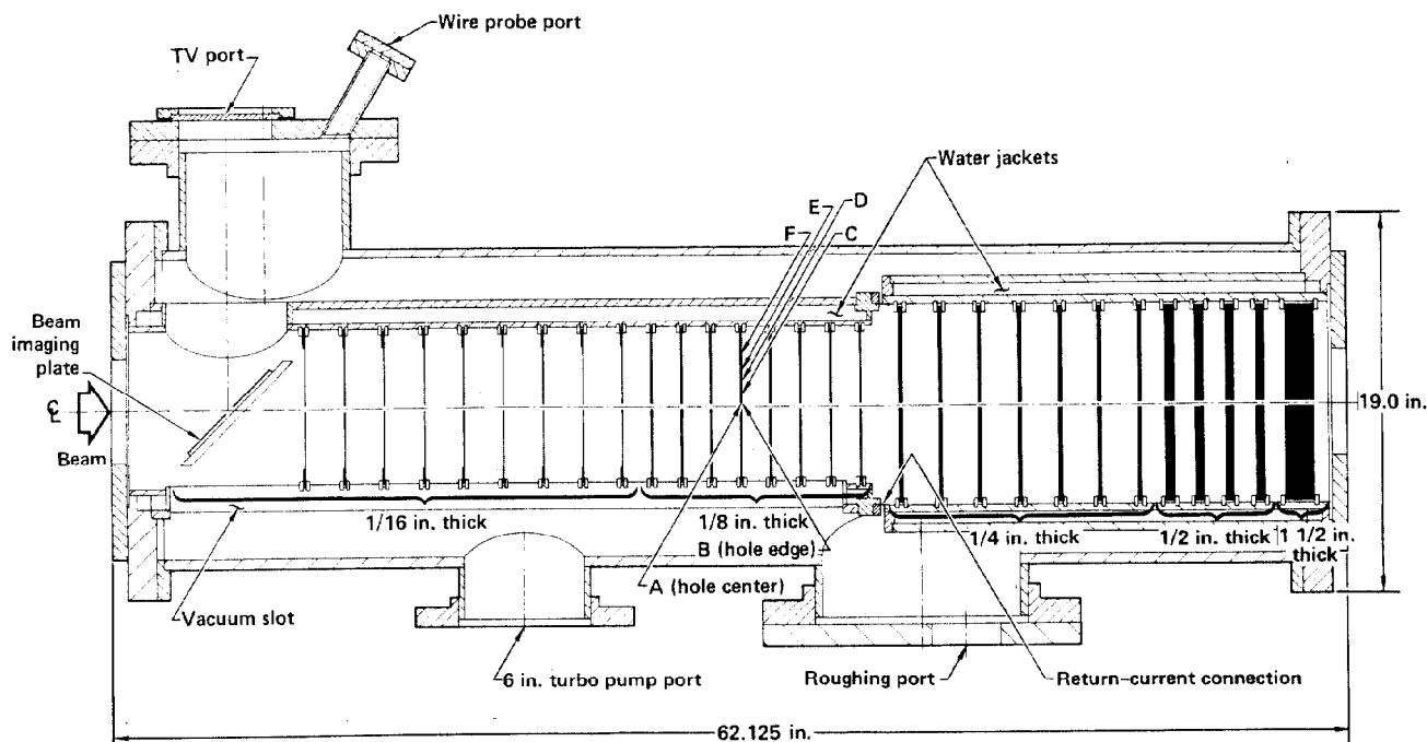
ATA Beam Dump/Emittance Box
