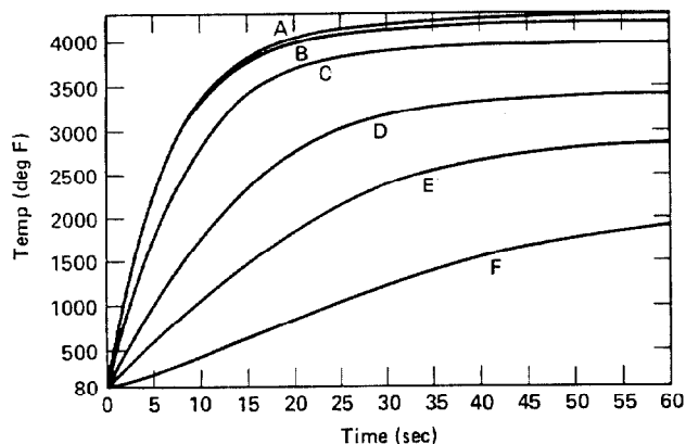
1/8 in. Thick Disks, 1 1/2 in. on Center
