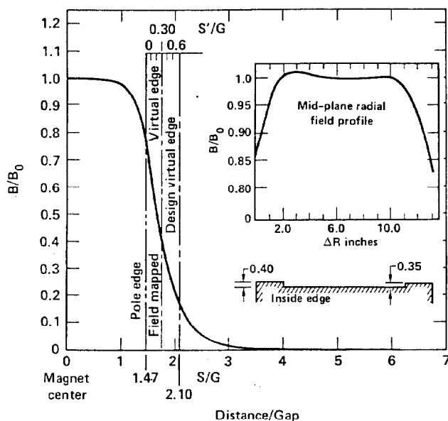
60° Analyzing Magnet Field Profiles
