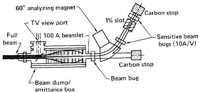
Beam Dump/Diagnostic Assembly
