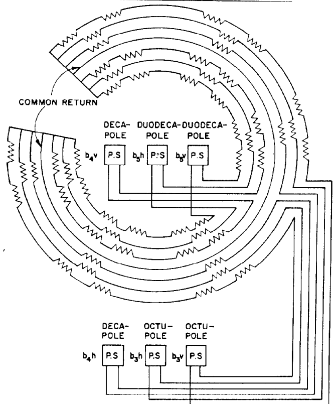
FIG. 3 MULTIPOLE CORRECTION CIRCUITS
