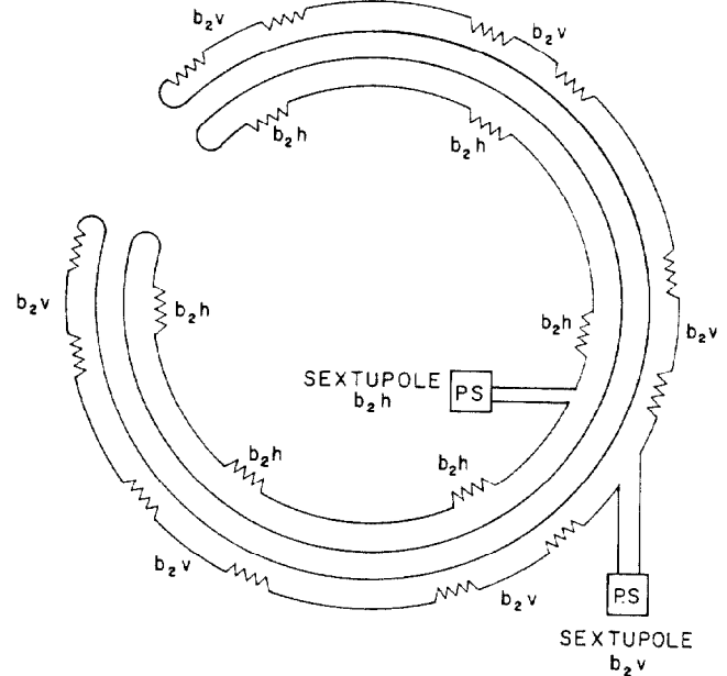
FIG. 2 SEXTUPOLE CORRECTION CIRCUITS
