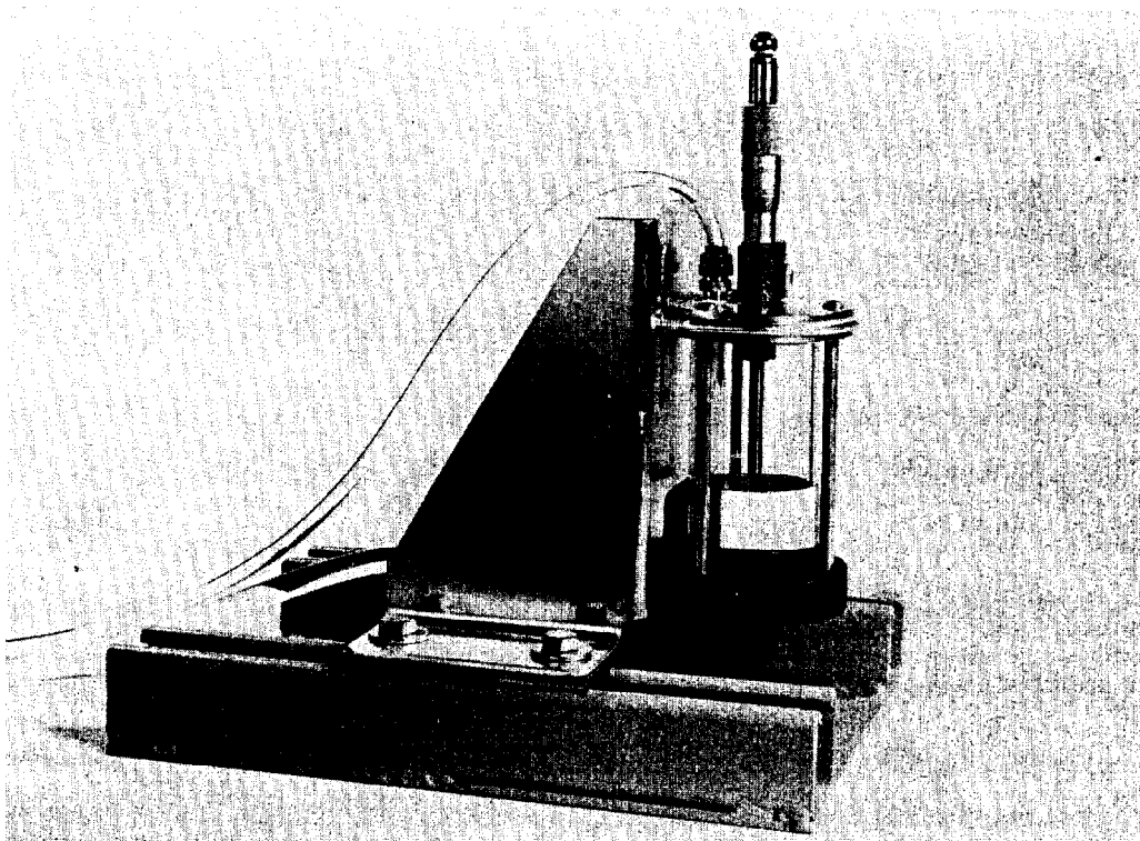
Figure 1. PEP Liquid Level "Well" with Support Stand
