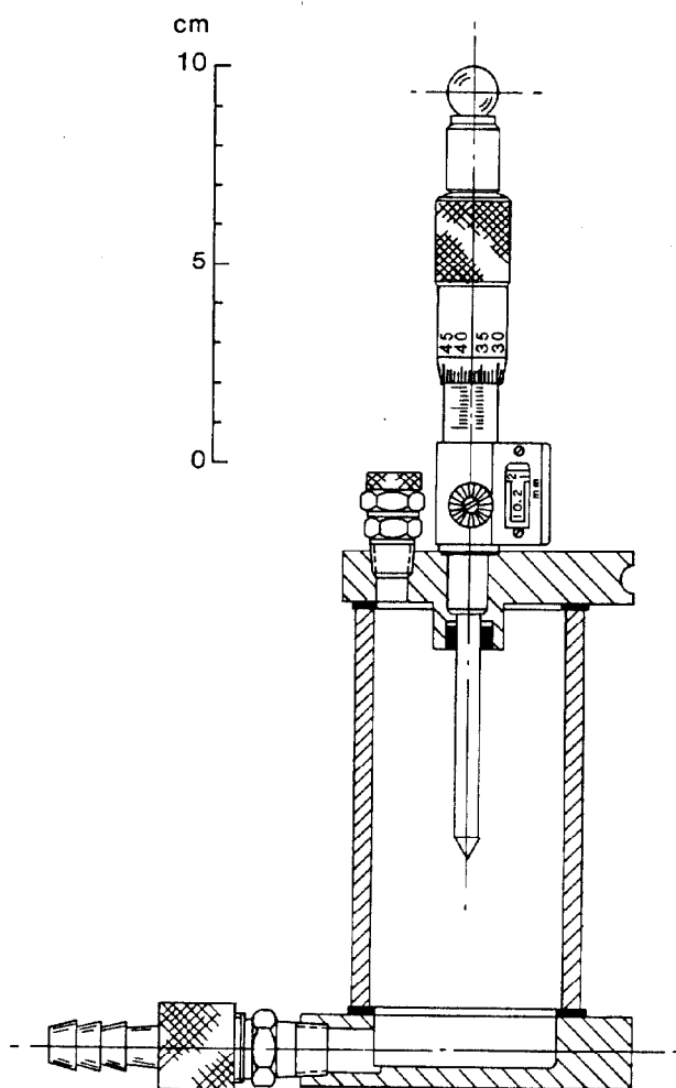
Figure 1. PEP Liquid Level "Well" with Support Stand
