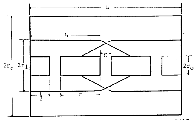
Fig. 2 L = 3/2 \beta\lambda Cell
