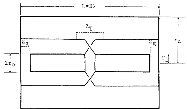
Fig. 1 L = \beta\lambda Cell
