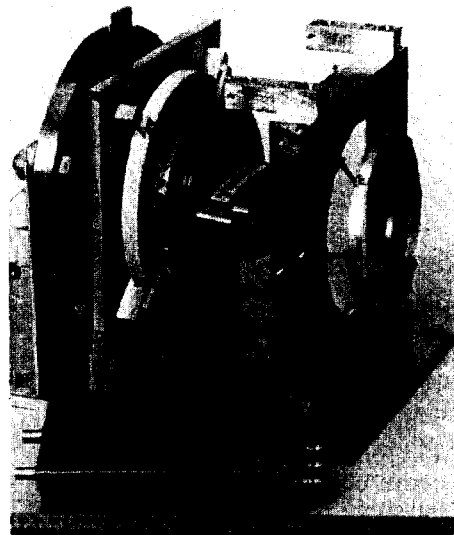
Fig. 4: Pickup-sensor with vacuum-section and preamplifier (housing removed)
