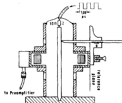
Fig. 5 Setup for alignment and calibration
