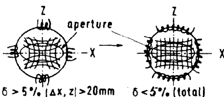
Fig. 3: Linearization of field pattern distortions
