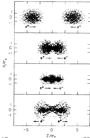
Fig. 5. Side view of the collision of oppositely charged beams, showing the pinch effect for Gaussian profiles and a disruption factor D = 14.4 .
