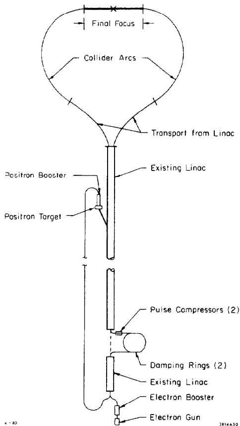
Fig. 1. General layout of the SLAC Collider.
