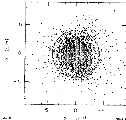
Fig. 3. A scatter plot of 3000 rays traced through the final focus system.
