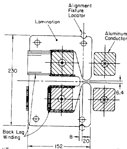
Fig. 2. Cross section of the SLC arc magnets. Dimensions are in millimeters.
