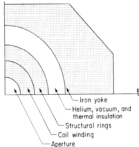
Fig. 1. Computer-generated quarter cross-section of base-case magnet for parameter study.
