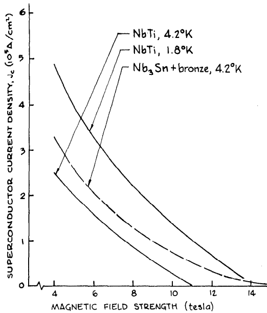
Fig. 4. Critical current density vs. magnetic field and temperature for various superconductors.
