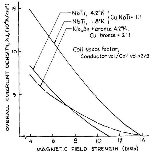
Fig. 5. Overall coil current density vs. magnetic field and temperature.
