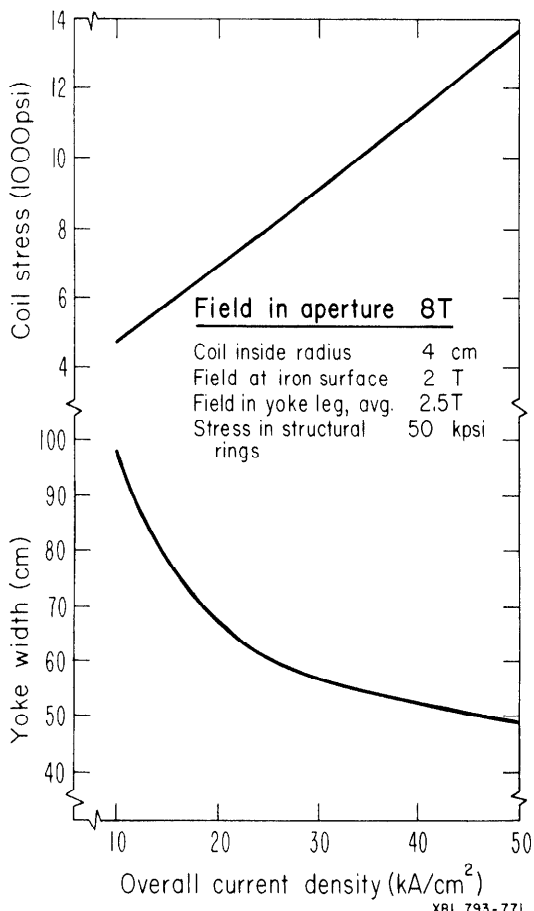
Fig. 2 and 3. The effects of magnetic field in the aperture and coil current density on the overall width and maximum coil compressive stresses.
