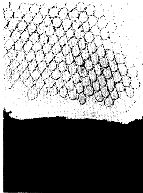
Fig. 4. Magnet braid to braid enlargement showing glass fibers and the multifilament superconductor
