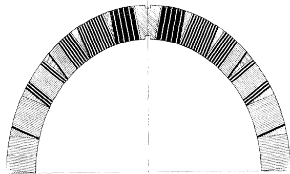
Fig. 1. The turns distribution utilized in the standard ring magnet dipole. One pole is shown here.
