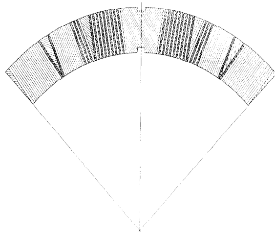
Fig. 2. The turns distribution utilized in the standard ring magnet quadrupole. One pole is shown.
