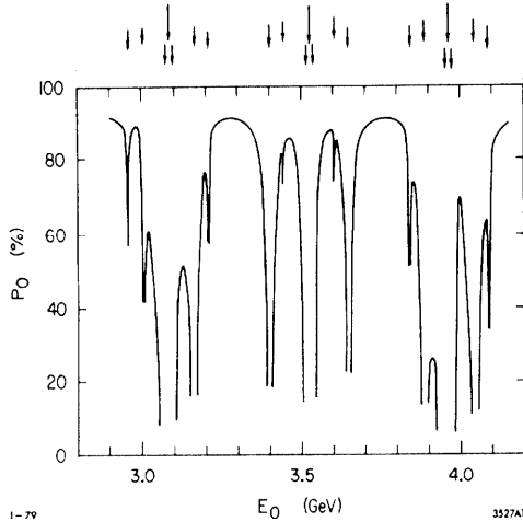
Fig. 1. A typical example for SPEAR showing the expected polarization P_0 versus the beam energy E_0 .
