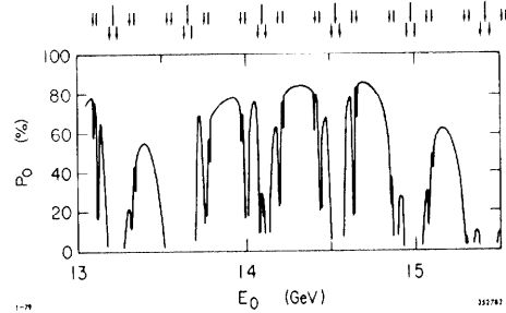
Fig. 2. A typical example for PEP showing the expected polarization P_0 versus the beam energy E_0 .
